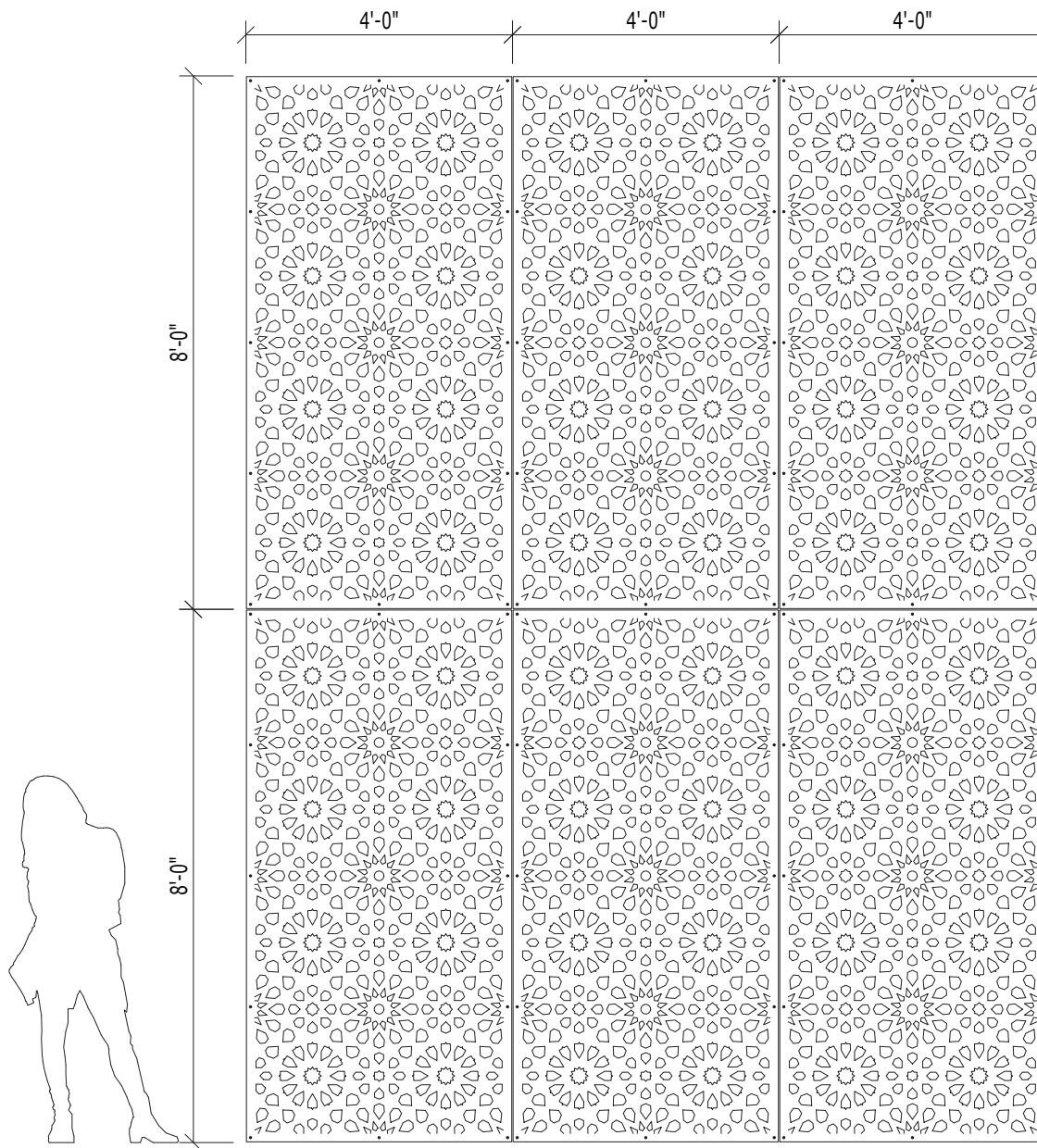
WALL SYSTEM WITH 4'-0" x 8'-0" STANDARD PANELS
