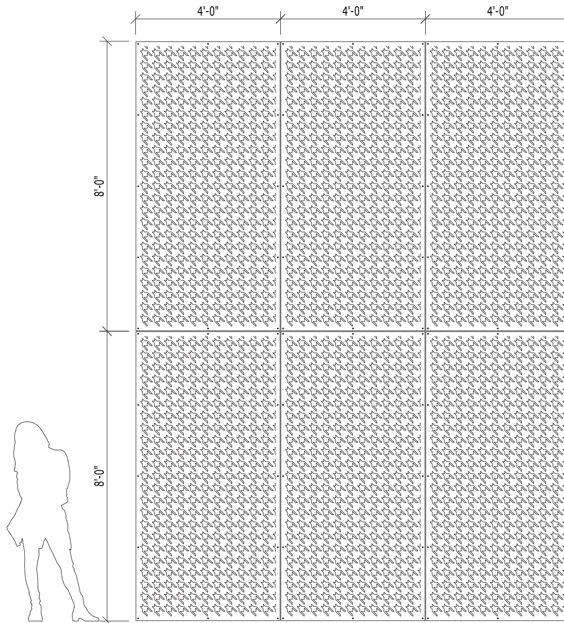
WALL SYSTEM WITH 4'-0" x 8'-0" STANDARD PANELS
